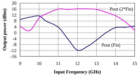
P_{out} = f(Fin) for P_{in}=12\text{ dBm} .
