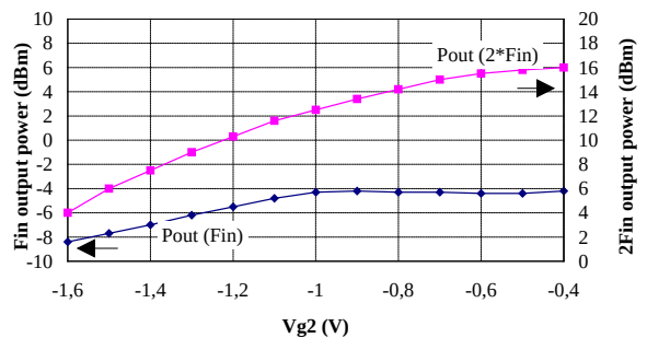
P_{out} = f(V_{g2}) for P_{in}=14\text{ dBm} and F_{in} = 11.5\text{ GHz}
