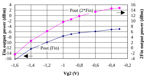
P_{out} = f(V_{g2}) for P_{in} = 10\text{ dBm} and F_{in} = 11.5\text{ GHz}
