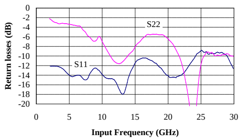
S_{11} and S_{22} = f(Fin) for P_{in} = 0\text{ dBm} .
