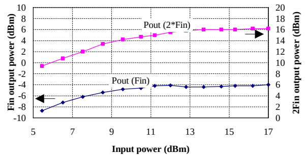
P_{out} = f(P_{in}) for F_{in} = 11.5\text{ GHz} .
