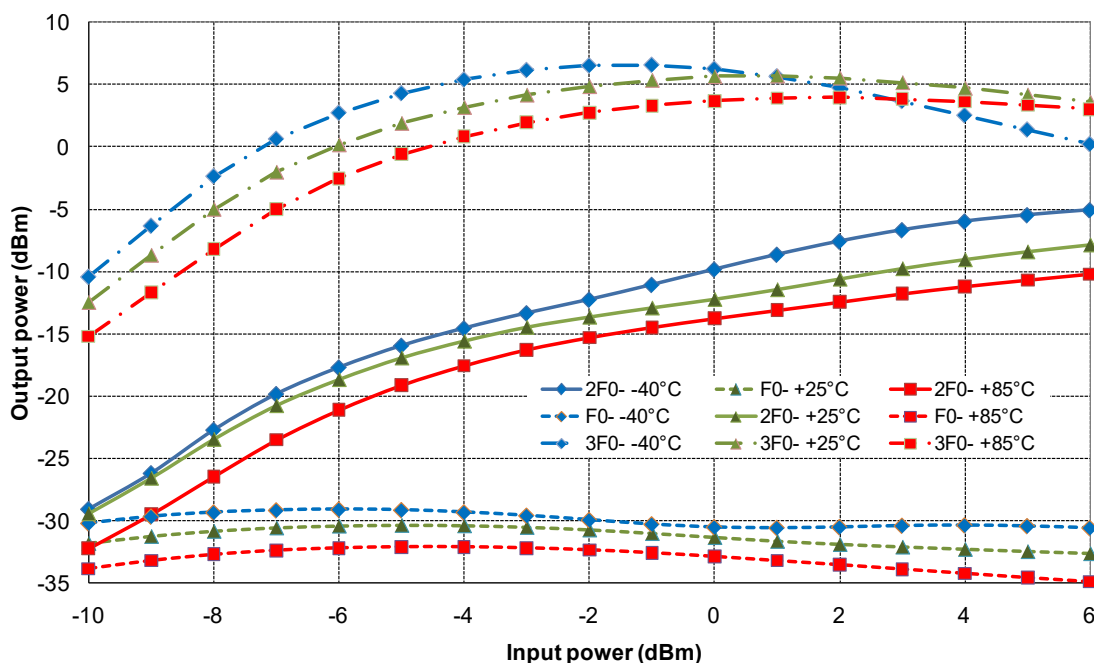
Harmonic output power vs. input power F 0 =12.5GHz
