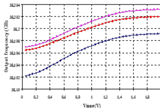
Typical tuning characteristic
