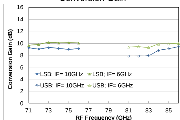
Conversion Gain
