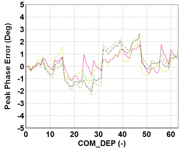
Peak phase error (deg) versus Phase State
