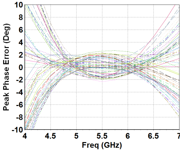
Peak phase error (deg) versus frequency All Phase States, one chip
