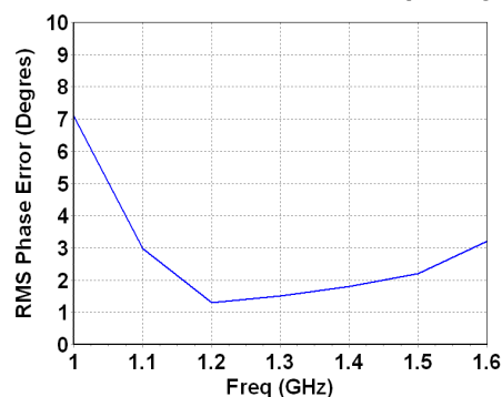
RMS Phase Error versus Frequency
