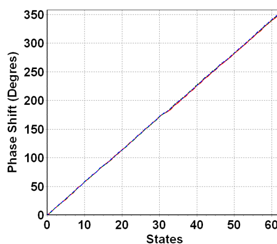
Phase Shift versus States (1.2 GHz ≤ Frequency ≤ 1.4GHz)
