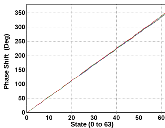
Phase shift versus state 2.7GHz < frequency < 3.4GHz
