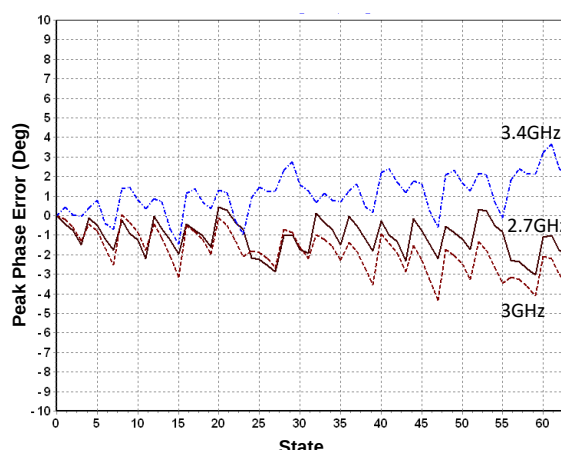
Peak Phase Error vs State @ 2.7, 3, 3.4GHz (packaged device, board measurement)
