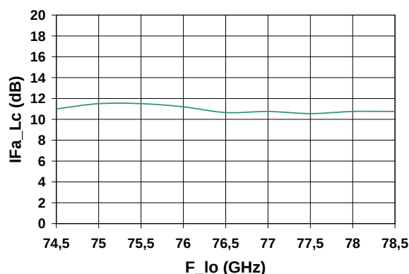
On wafer typical IFa_Lc measurement
