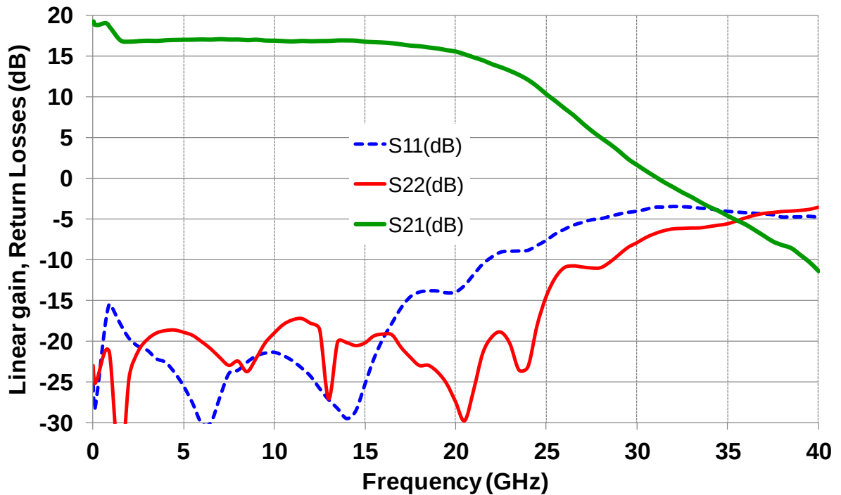
Broadband Linear Gain and Return Losses vs. frequency
