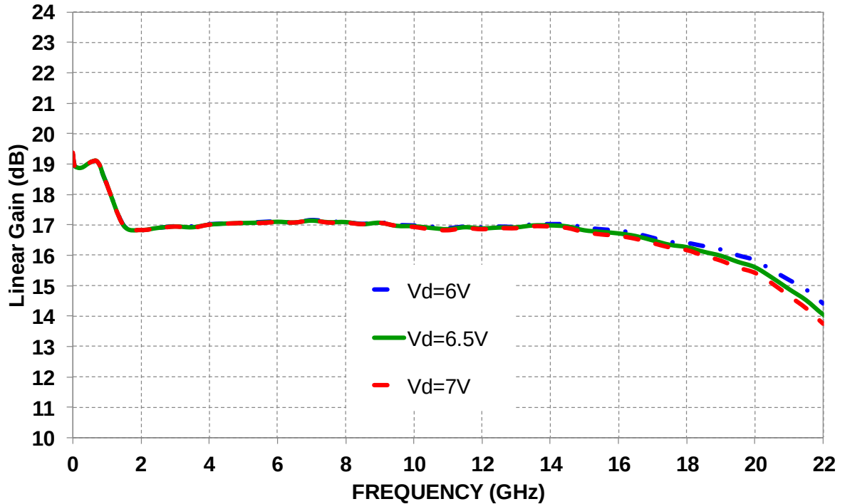
Linear Gain vs. Frequency and Vd
