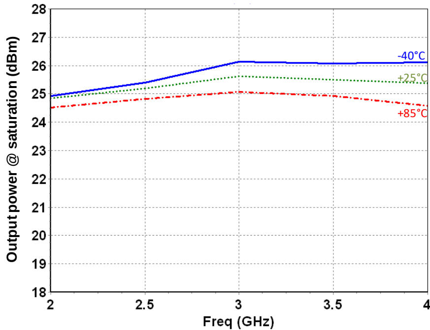
Output power @ saturation versus Frequency &amp; Temperature
