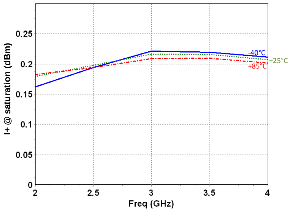
Positive supply current @ saturation versus Frequency &amp; Temperature
