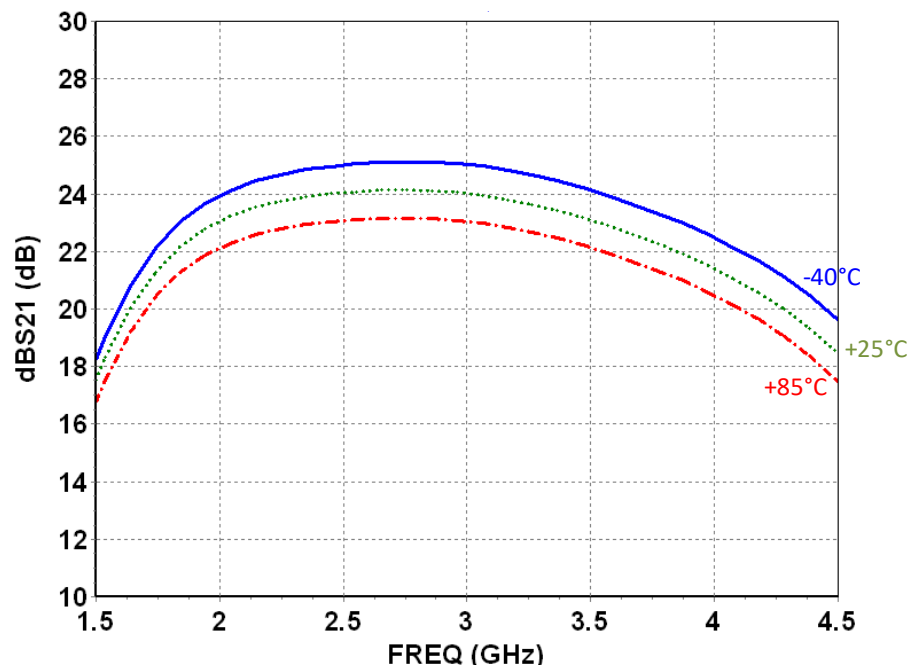
Linear Gain
