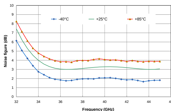
Noise figure versus temperature
