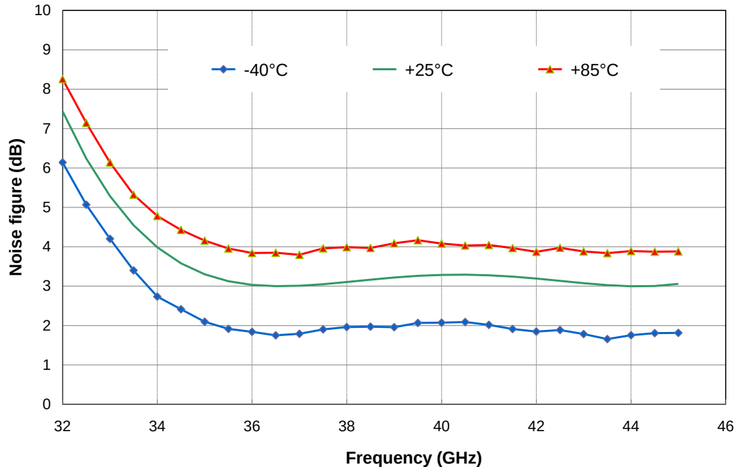
Noise figure versus frequency &amp; temperature
