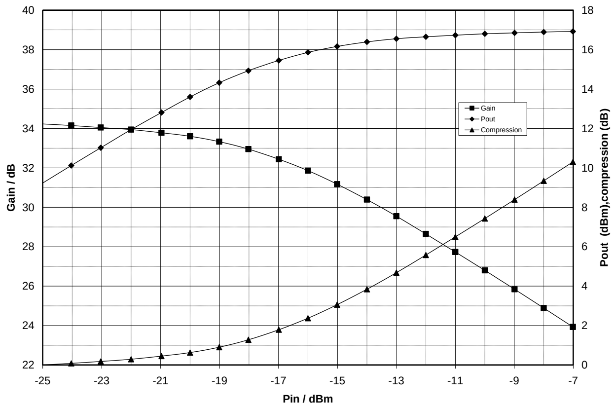
Gain / Pout @ 16GHz
