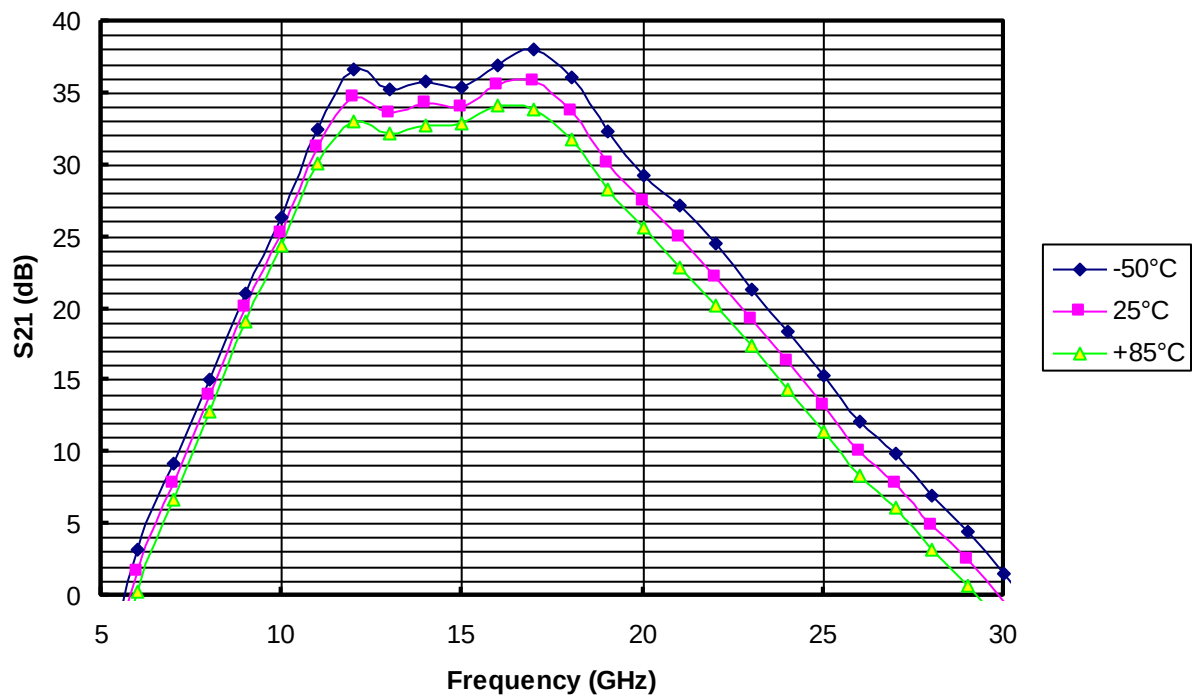
S21 in the full temperature range
