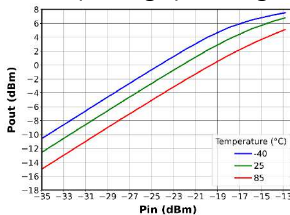
Pout vs Pin and Temperature @Idq = 30mA & @ Freq = 28GHz
