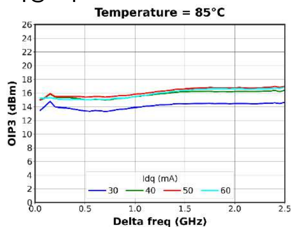
OIP3 vs Delta Freq and I_{dq} @Freq = 27.75GHz
