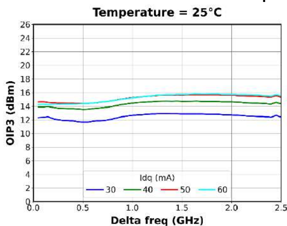
OIP3 vs Delta Freq and I_{dq} @Freq = 25.25GHz
