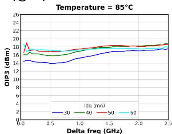
OIP3 vs Delta Freq and I_{dq} @Freq = 30.25GHz
