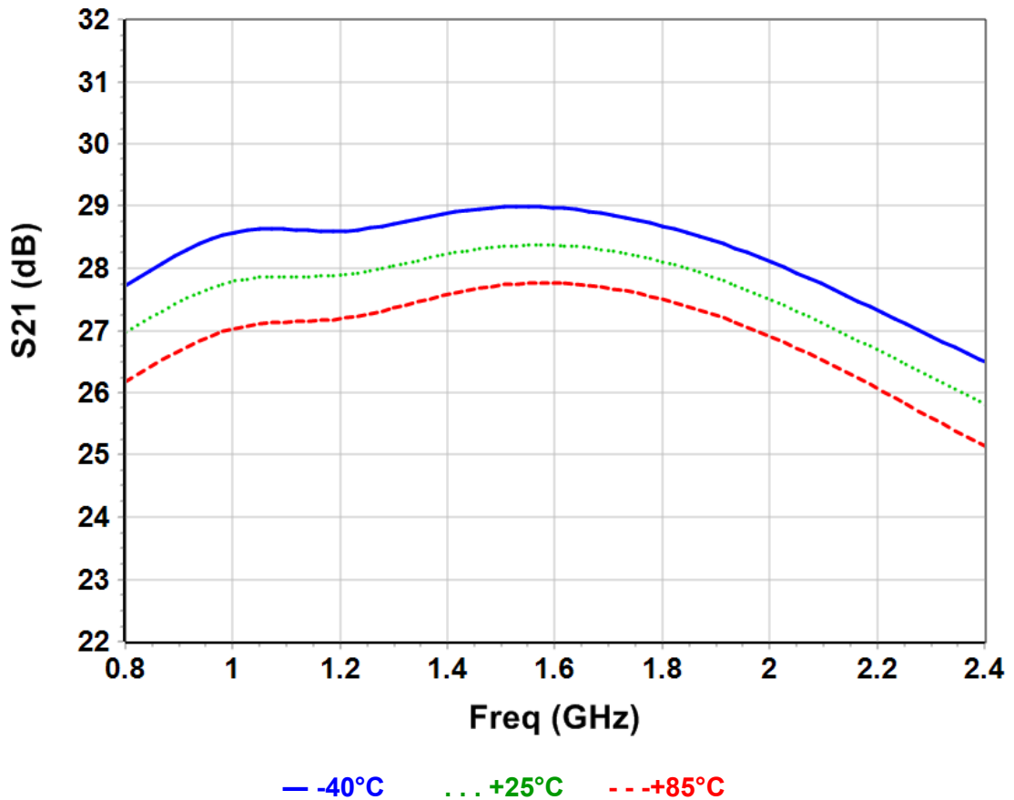
Linear Gain vs. Frequency
