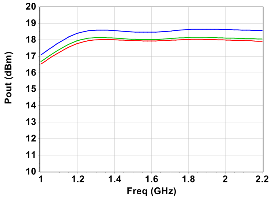
Output power @ Sat vs. Frequency
