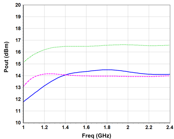
Output power @ 1dB comp. vs. Frequency
