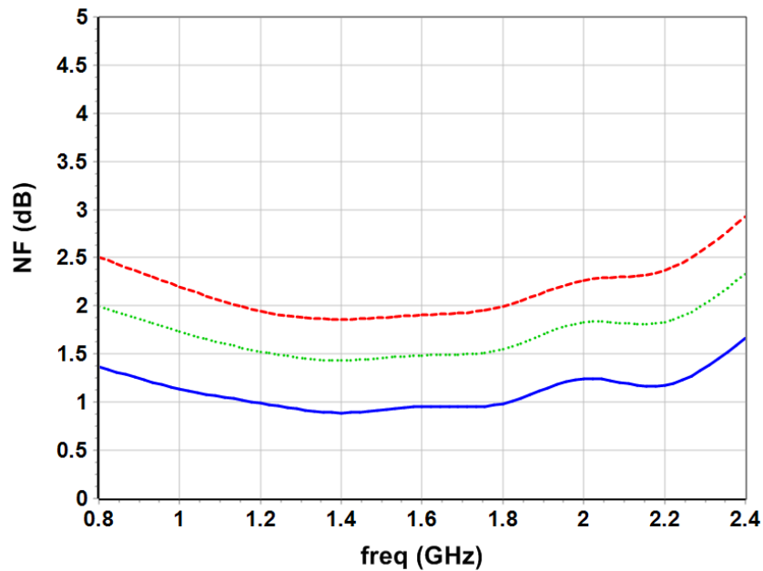
Noise Figure vs. Frequency
