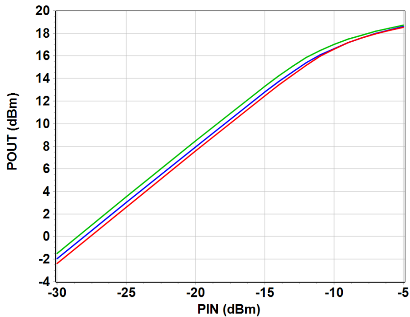
Output power vs. Input Power @ 25°C
