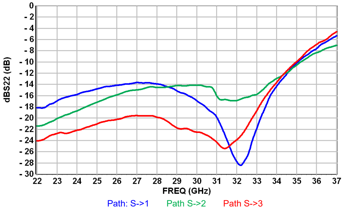
Output Return Loss (Port 1,2,3) versus Frequency
