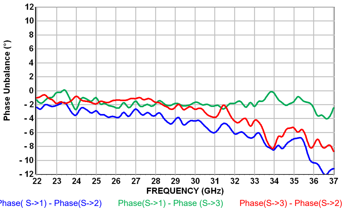
Phase Unbalance versus Frequency
