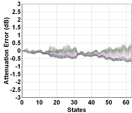
Attenuation Error versus States 0.5GHz < Frequency < 6GHz
