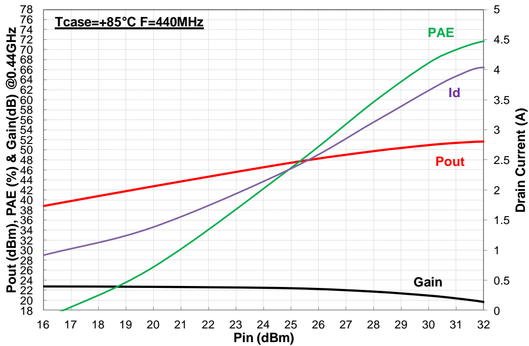
Pout, PAE, Gain & Id @ Freq = 440MHz & Tc = +85°C
