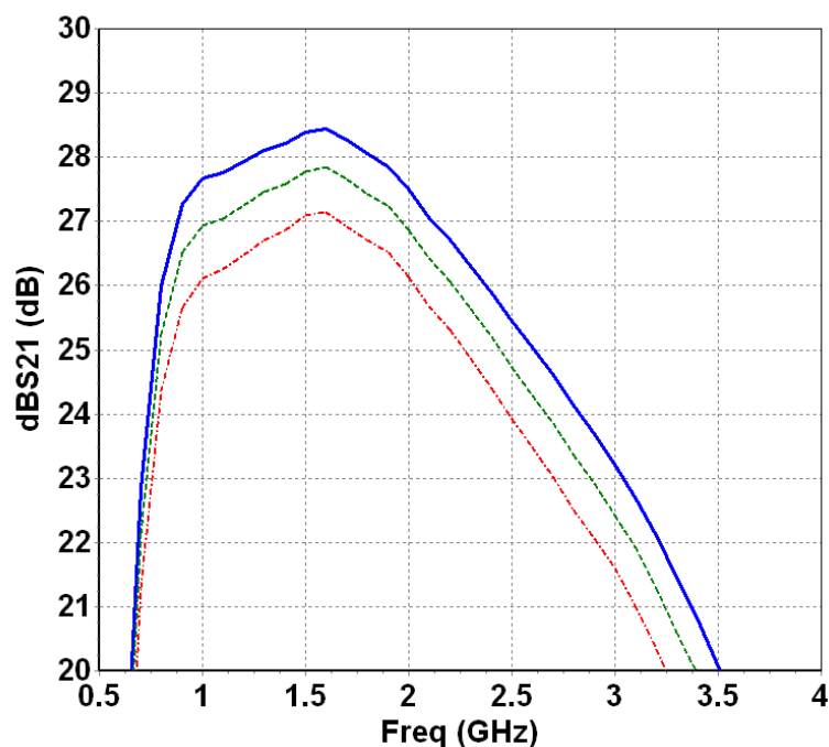
Linear Gain vs. Frequency
