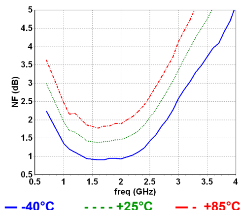
Typical Noise Figure vs. Temperature
