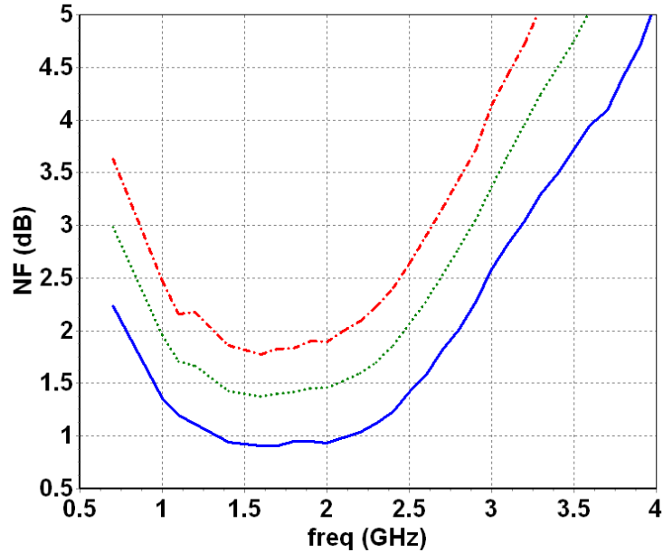
Noise Figure versus Frequency
