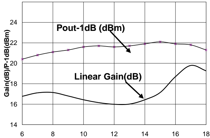
Gain and Output power Versus input power & Frequency Test fixture measurement
