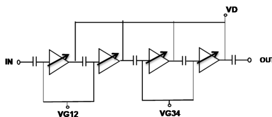
Functional diagram
